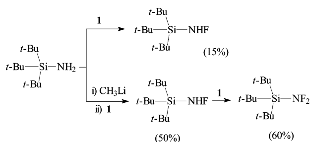
Scheme 12
