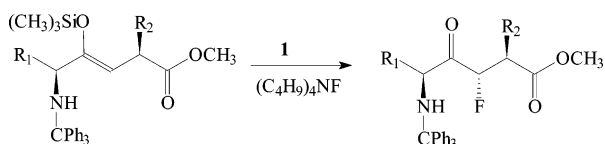
Scheme 24
